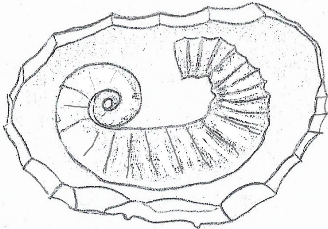
amonit
