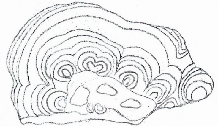
malachit
